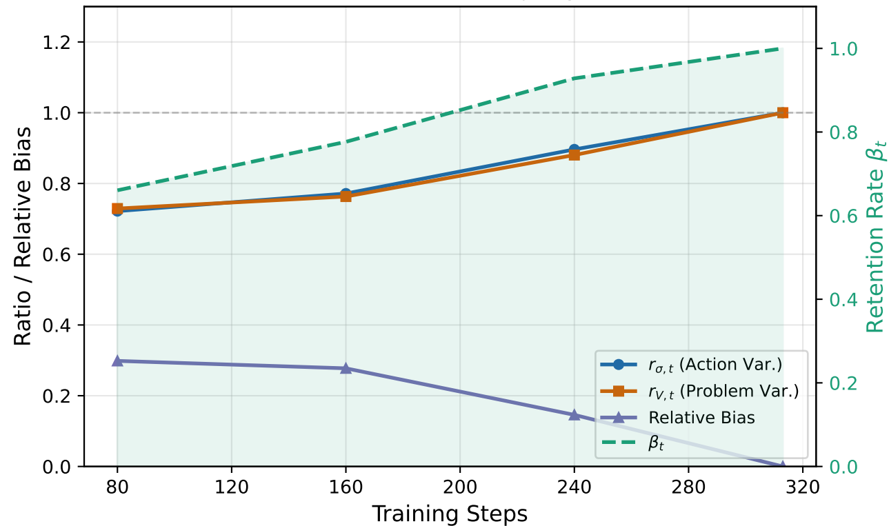
Qwen2.5-Math-1.5B (Majority Vote)
